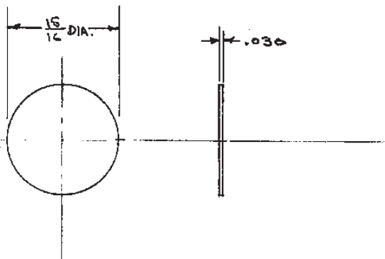
# 4620 DIAPHRAGM (NYLON)
